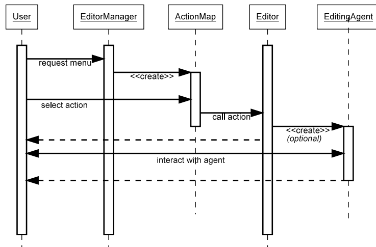
Figure 12: Sequence of operations involving the editor manager.
