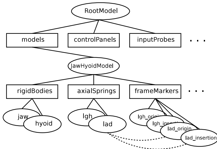
Figure 4: A partial component hierarchy for a Jaw-Hyoid model. The dashed lines show the references from the muscle lad to its two attachment markers (other references are omitted for clarity).
