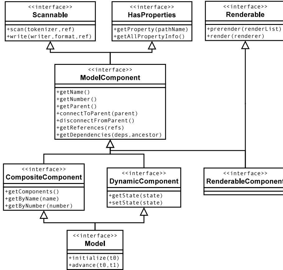
Figure 3: Basic ArtiSynth component classes.
