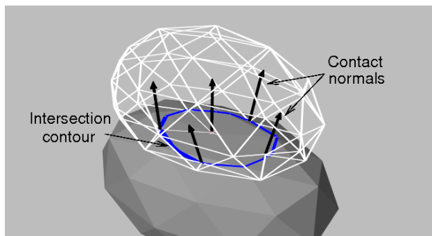
Figure 15: Contact handling between two deformable models (with the topmost rendered as a wireframe), showing the intersection contour (blue) and the contact normals (black lines) of interpenetrating vertices from the upper mesh.
