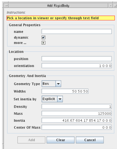
Figure 13: Editing agent dialog for adding rigid bodies.
