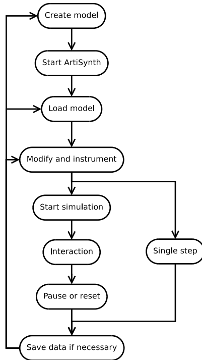
Figure 6: Typical ArtiSynth usage sequence.
