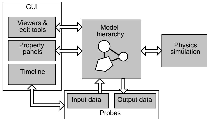
Figure 2: General organization of the ArtiSynth system.
