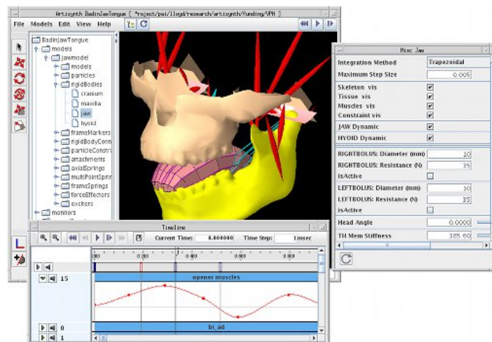
Figure 1: ArtiSynth screen shot showing a combined jaw-tongue-hyoid model, with the main viewing panel (center), component navigation panel (left), probes arranged on the timeline (bottom), and a panel for adjusting properties (right).
