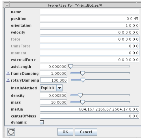
Figure 11: Property editing panel for a rigid body.
