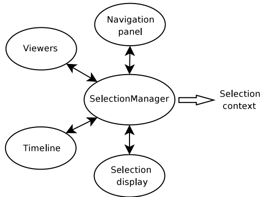
Figure 8: The ArtiSynth selection manager.
