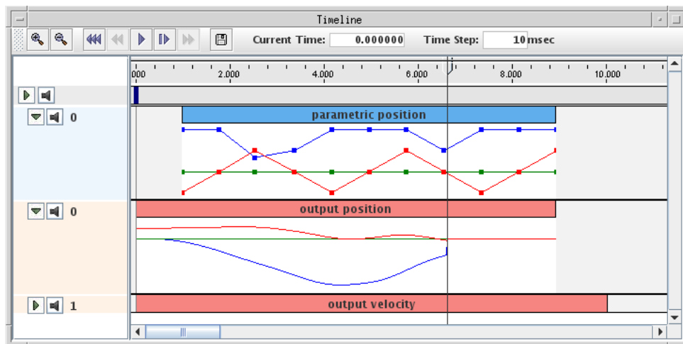
Figure 14: Timeline with probes expanded to show data.
