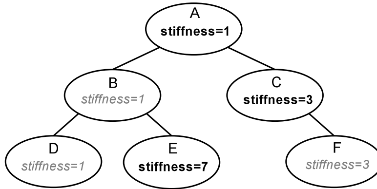
Figure 5: Inheritance of a property named stiffness among a component hierarchy. Explicit settings are in bold; inherited settings are in gray italic.
