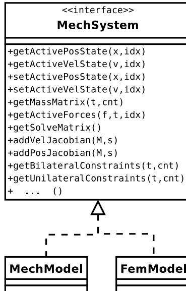
Figure 16: Top-level ArtiSynth mechanical models must implement MechSystem , shown partially here.
